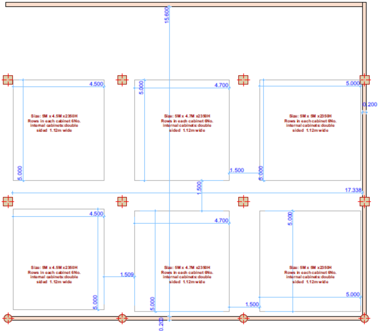
TYPICAL LAYOUT FOR BULK FILERS
